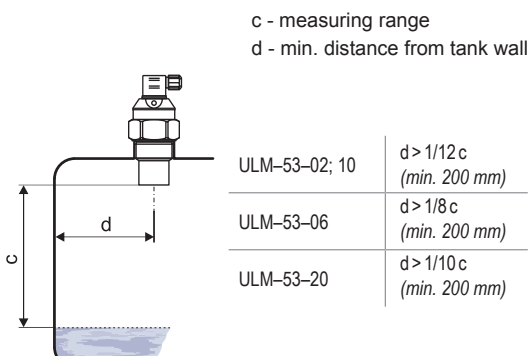
Installation distance from the tank wall
