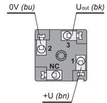
The inside of the connector socket
