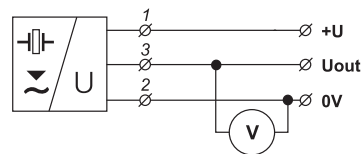
Connection scheme
