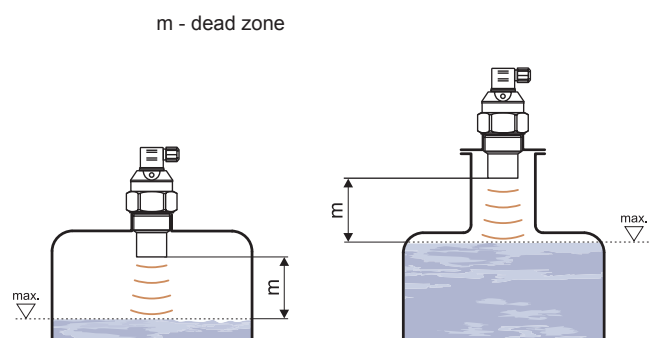
Maximum level distance from ULM
