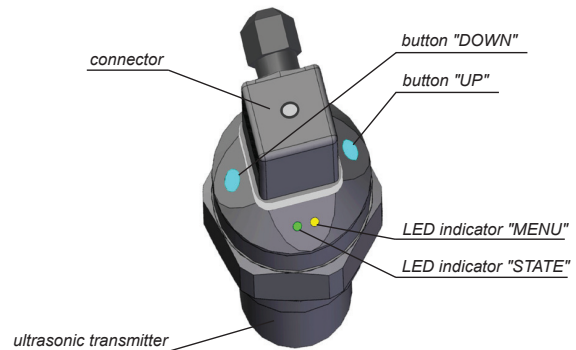
Full view of ultrasonic level meter
